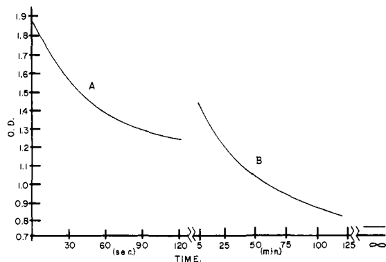
Fig. 1.—Acylation and deacylation of formohydroxamic acid with cinnamoylimidazole at 25° in phosphate buffer (0.05 M ), pH 6.86, 0.67% \text{CH}_3\text{CN} ; [\text{FHA}] = 2.33 \times 10^{-3} \text{ M} , [\text{CI}] = 1.00 \times 10^{-4} \text{ M} ; curve A, at 320 \text{m}\mu ; curve B, at 290 \text{m}\mu .
