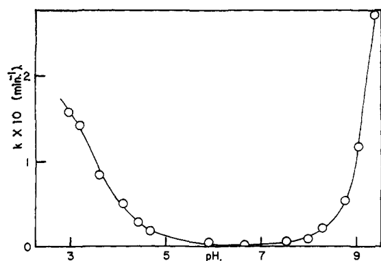
Fig. 6.—pH dependence of the hydrolysis of cinnamoylimidazole in 1.67% acetonitrile, 25°, \mu = 0.1 . The profile is very similar to that reported by Jencks and Carriuolo 8 : —, calculated for pK_{CIH}^+ = 3.66 and the kinetic parameters described in the text.
