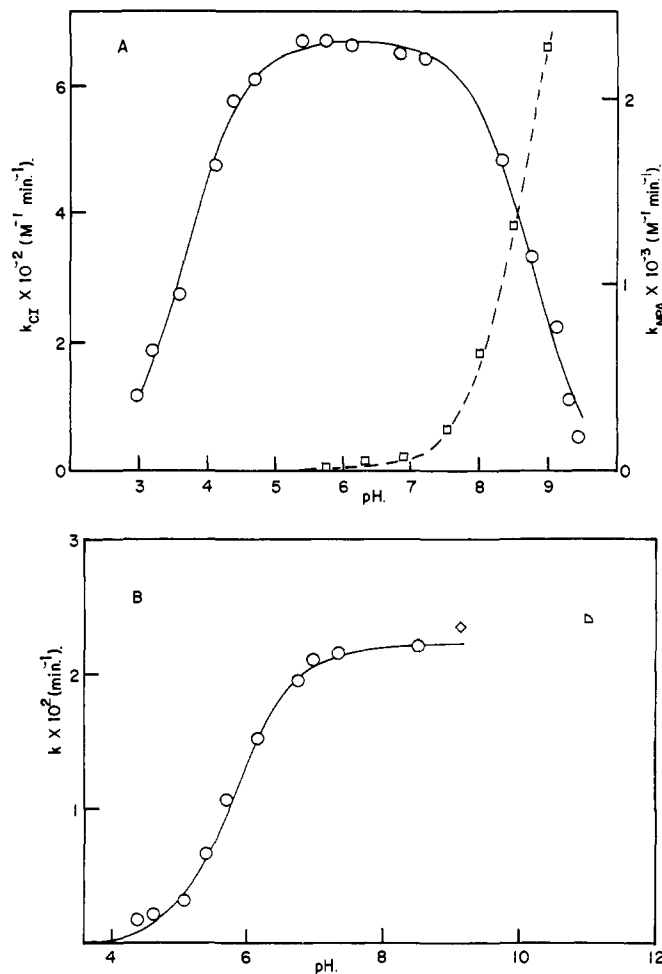
Fig. 2.—Dependence of specific rate of reaction on pH at 25° and \mu = 0.10 . A. Acylation reactions: —, acylation of FHA with cinnamoylimidazole, calculated for \text{p}K_{\text{CIH}^+} = 3.66 and \text{p}K_{\text{FHA}} = 8.70 ; - - - - - , acylation of FHA with p -nitrophenyl acetate, calculated for \text{p}K_{\text{FHA}} = 8.70 . B. Deacylation of the cinnamoyl intermediate: —, calculated for \text{p}K_A = 5.70 ; O, acetate, phosphate, and pyrophosphate buffers ( \mu = 0.1 ); ◇, tris buffer; D, carbonate buffer.
